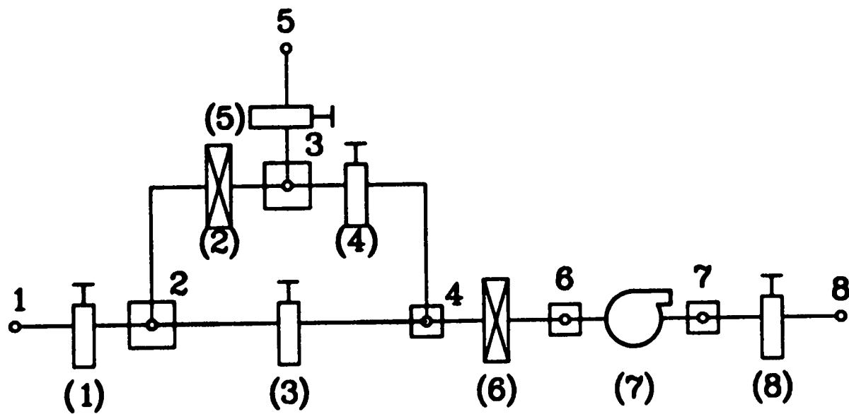
Fig. 10(a). FIRAC model of the simple flow network with leak path using standard nodding.
