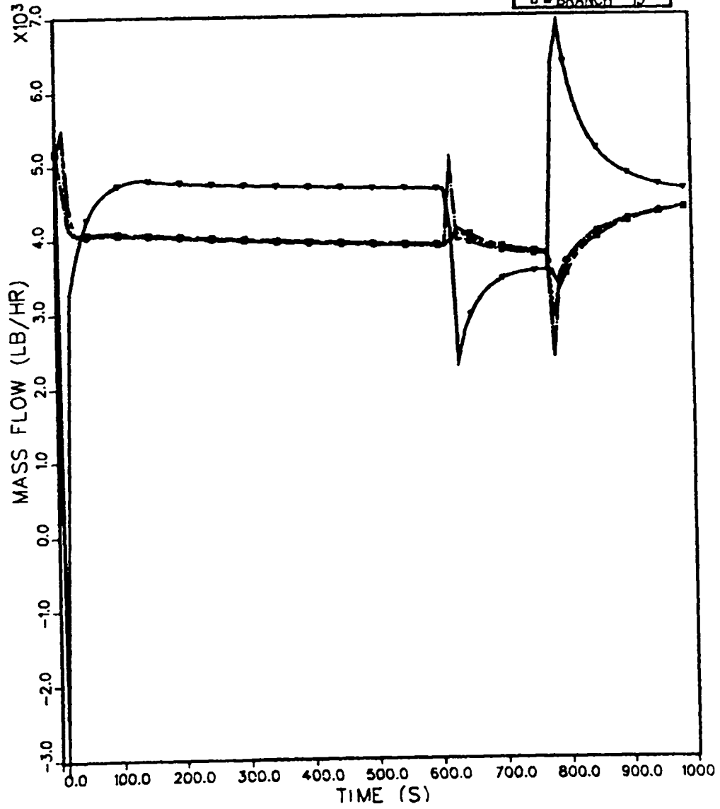
Fig. 20. Mass flow rates for branches 2, 3, 8, and 15.
