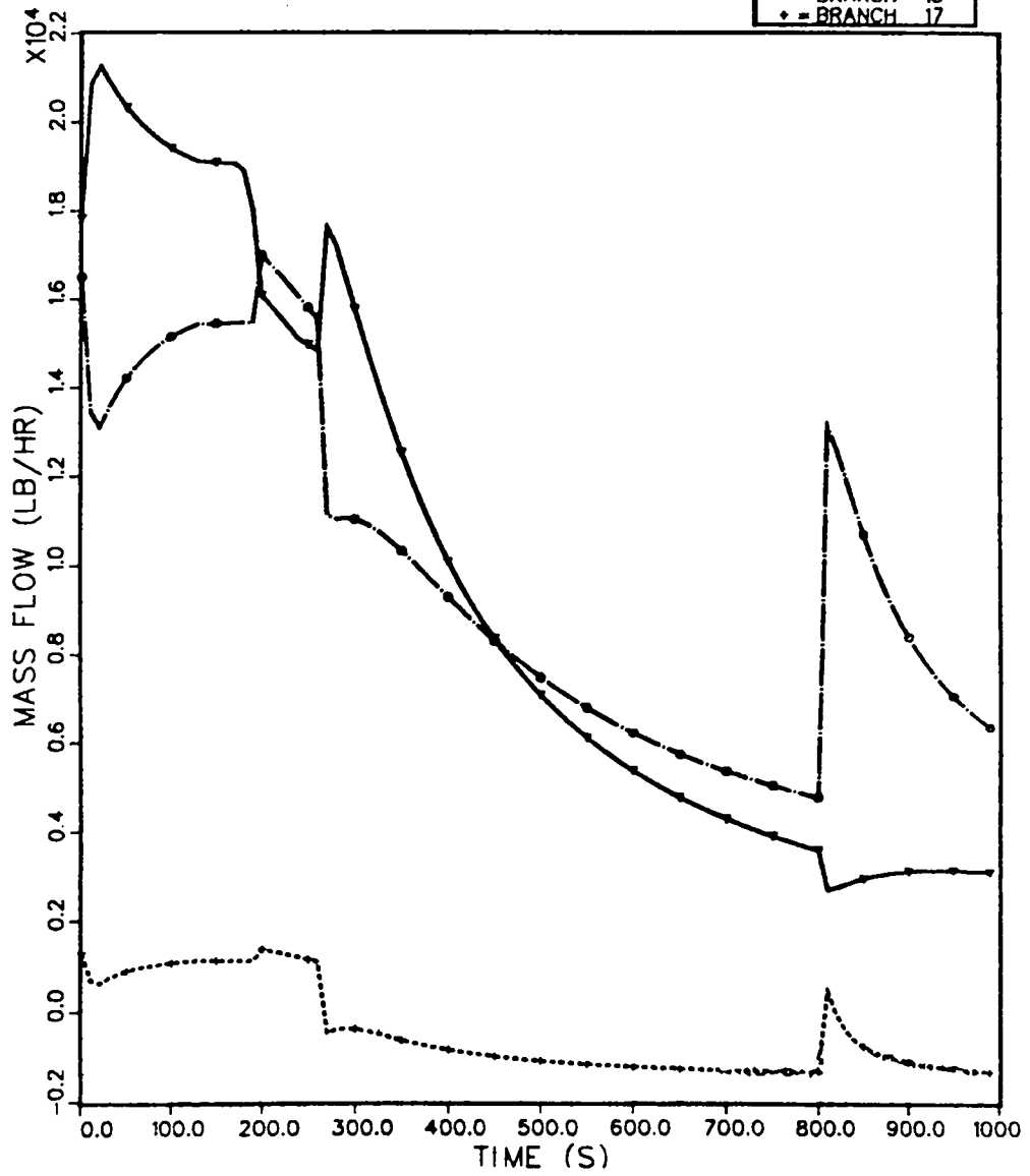
Fig. 34. Fire compartment mass flow rates (branches 14, 16, and 17).
