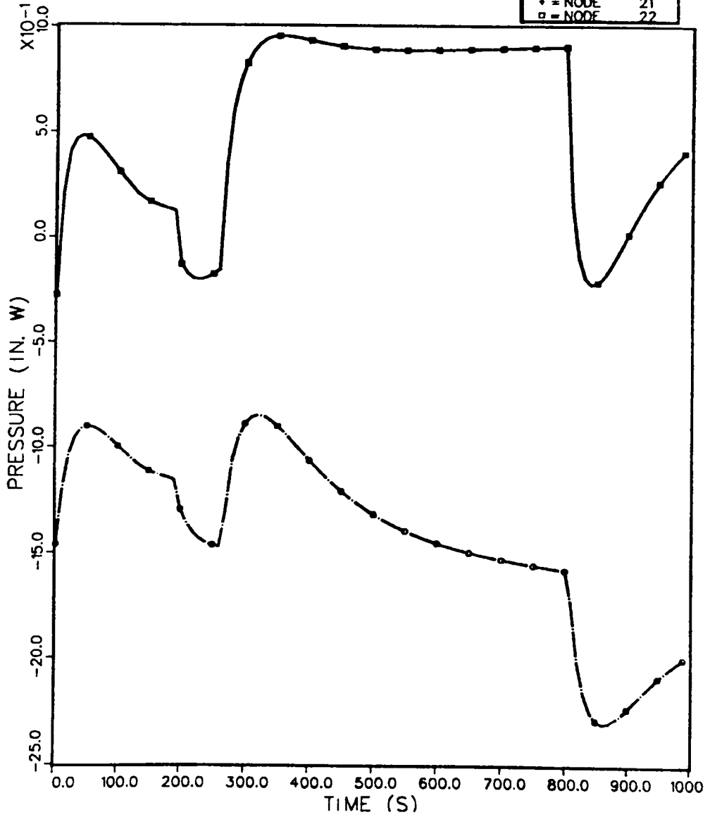
Fig. 32. Pressure response for nodes 9, 15, 21, and 22.
