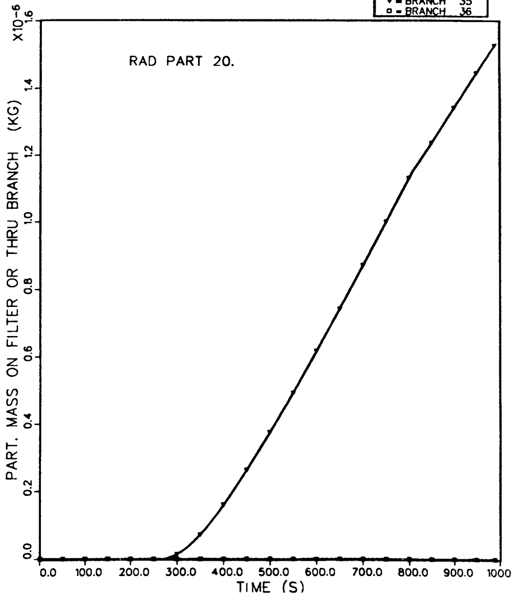
Fig. 44. 20-µm radioactive particulate mass for branches 14, 34, 35, and 36.
