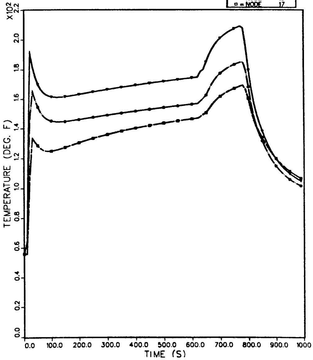
Fig. 24. Temperature response for nodes 9, 14, 16, 17.
