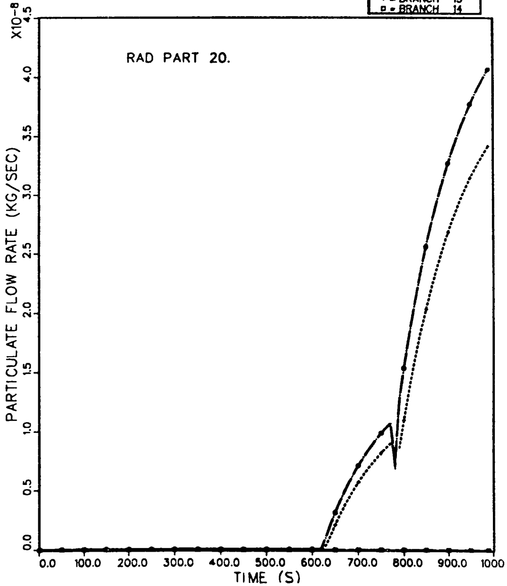
Fig. 29. 20- \mu m radioactive particulate mass flow rates for branches 2, 3, 13, and 14.
